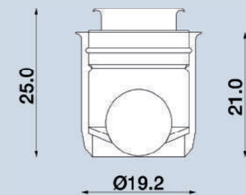
Stem Ø19,2 (bottle mouth Ø18,5mm)
