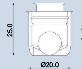
Stem Ø20 (bottle mouth Ø19mm)
